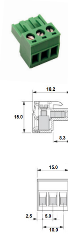
Screw terminals 45° angle
