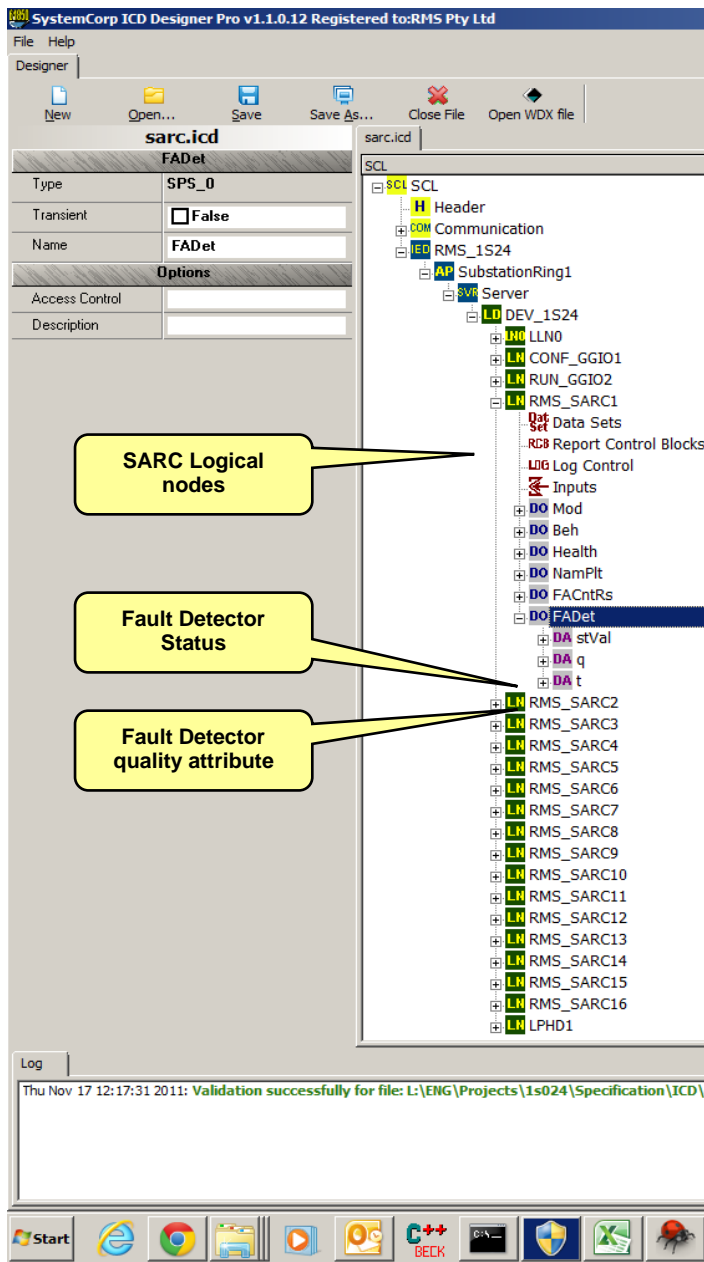
Figure 8: ICD editing screen
