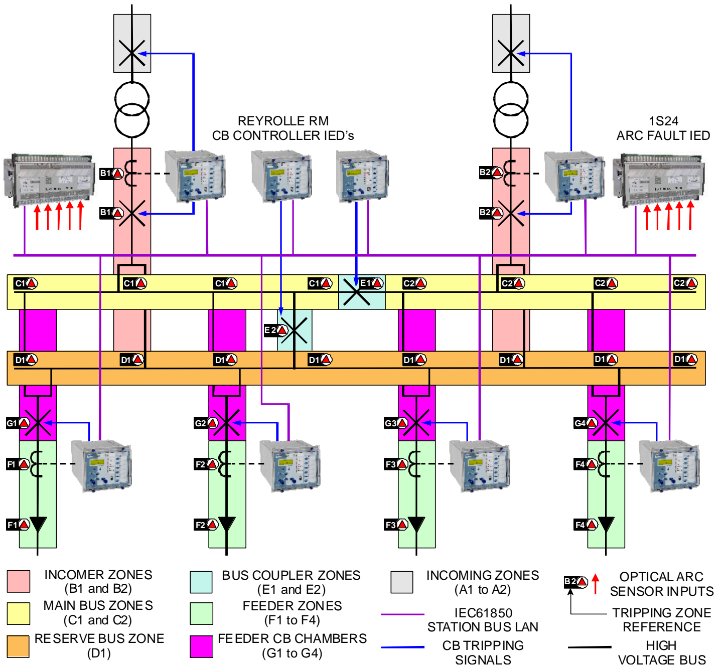
Figure 29: Double bus scheme 1S24/ J / 26/07/2022 - 12/25
