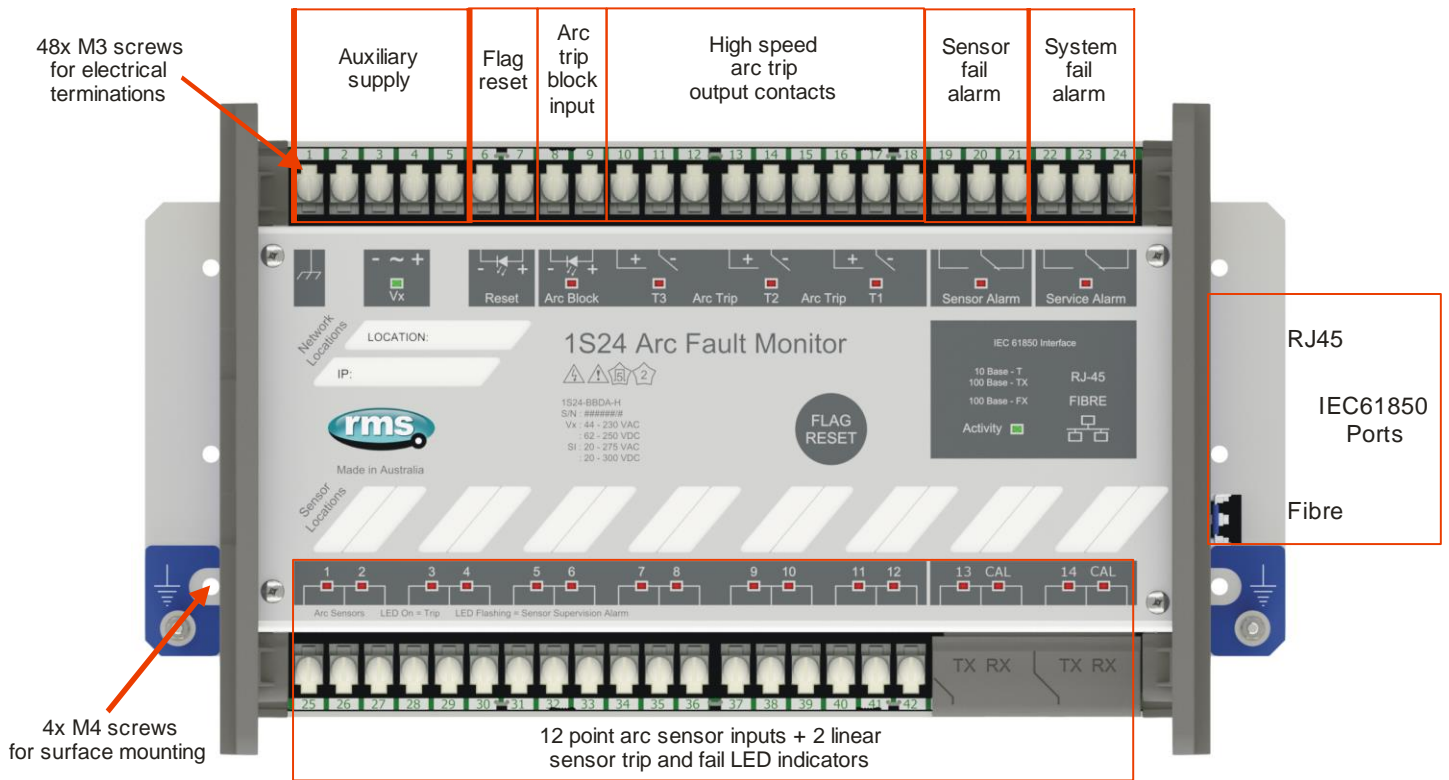
Figure 30: Front panel layout
