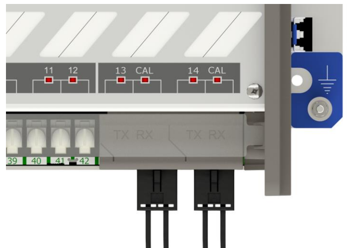
Figure 38: 1S40 Rx and Tx optic fibre connections
