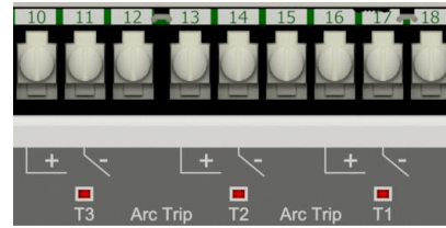
Figure 13: Arc trip output contacts and trip LED
