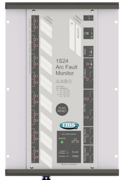
Figure 33: Vertical front panel layout
