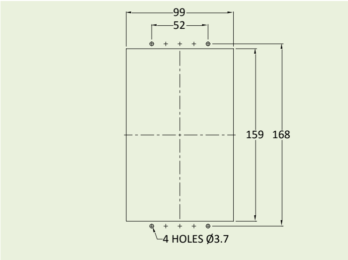
Panel Cut-out
