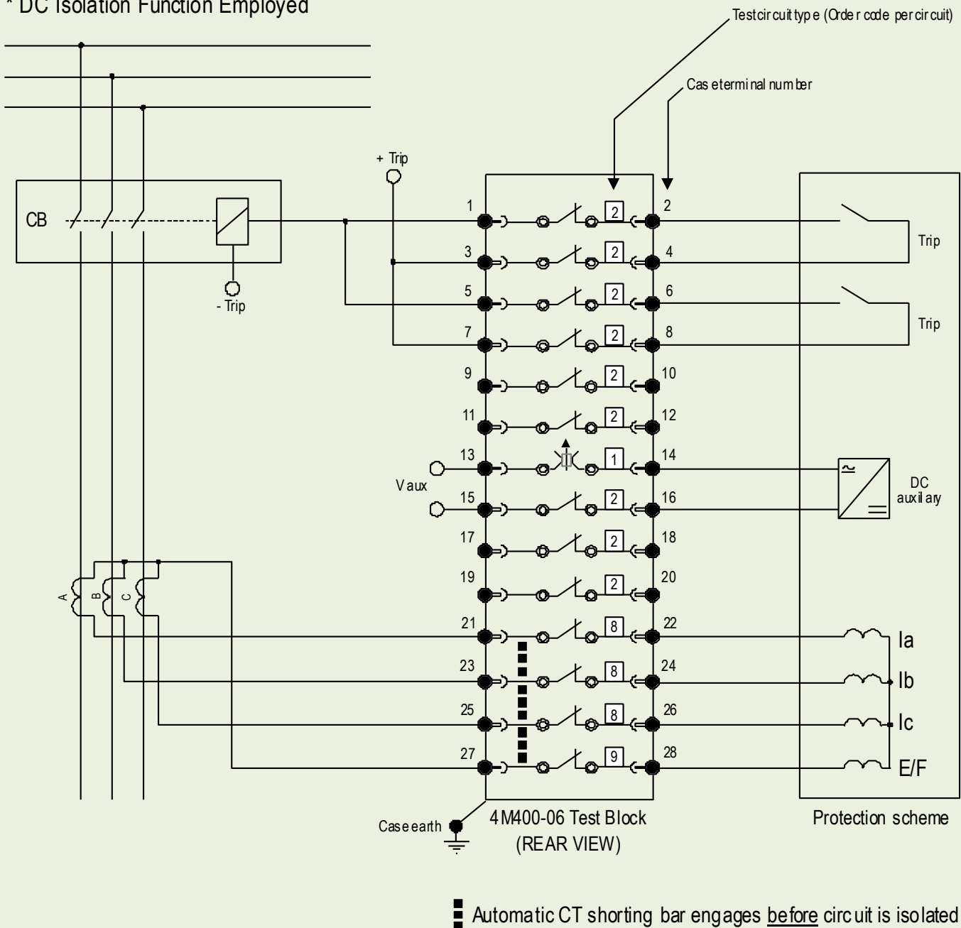
Figure 8: Application wiring example for a three phase overcurrent and EF protection scheme with auto CT shorting Viewed from rear terminal side
