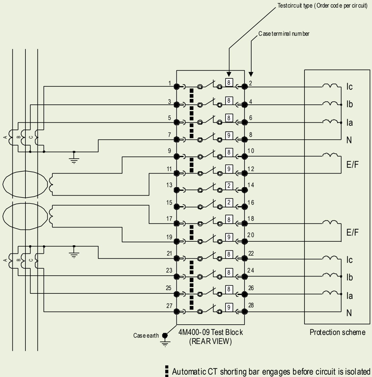
Figure 11: Application wiring example for differential protection of transformers with auto CT shorting Viewed from rear terminal side
