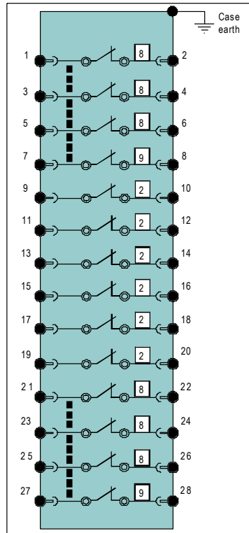
Figure 13: Viewed from rear terminal side Full order code: 4M400-S- 8 8 8 9 2 2 2 2 2 2 2 2 8 8 8 9 Short code: 4M400-22
