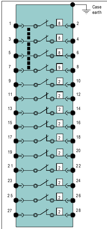
Figure 12: Viewed from rear terminal side Full order code: 4M400-S- 8 8 8 9 2 2 2 2 2 2 2 2 2 2 2 2 Short code: 4M400-21
